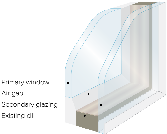
Fig. 10 – Secondary glazing
