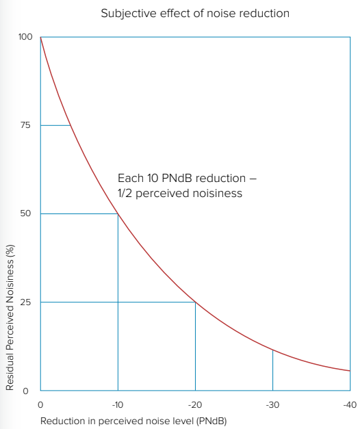
Fig 4 – Apparent loudness
