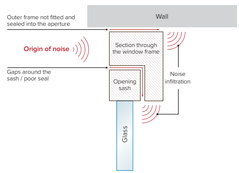
Fig 7 – Sound infiltration
